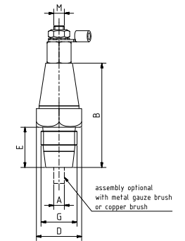
Design 3 spark plug holder
