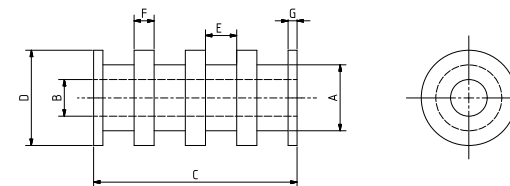
Spindle for U-bolt brush holders
