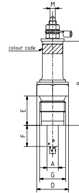
Design 1 telescope conductor with telescope gauze brush
